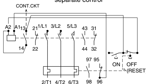
MS-N21~N35PM
