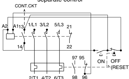
MS-N20PM
