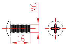
M6*16镀锌螺丝
